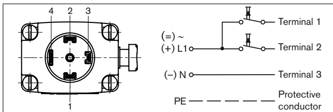
Fig. 4: Electrical connection - pulse model (CF 02)
